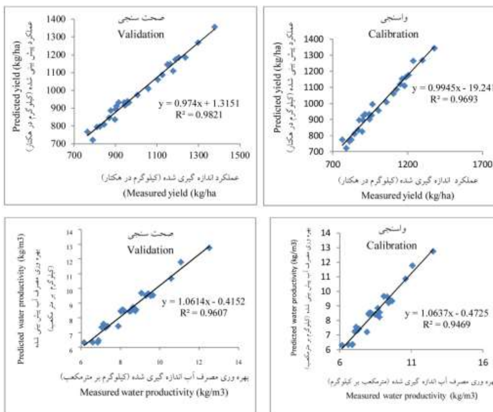
Figure 3. Measured and predicted values of yield and water productivity of quinoa under salinity, drought and Biochar conditions.
