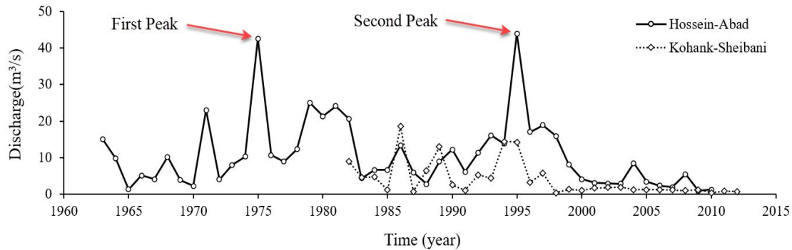
Figure 2. Annual time series graph of flow discharge at Hossein-Abad and Kohank-Shibani hydrometric stations in periods 1963-2010 and 1982-2012, respectively.
