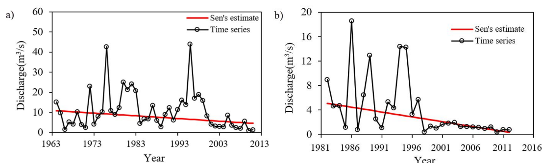
Figure 3. Investigating the trend of annual discharge using the Mann-Kendall test and Sens coefficient, a) Hossein-Abad station and b) Kohnek-Shibai station.
